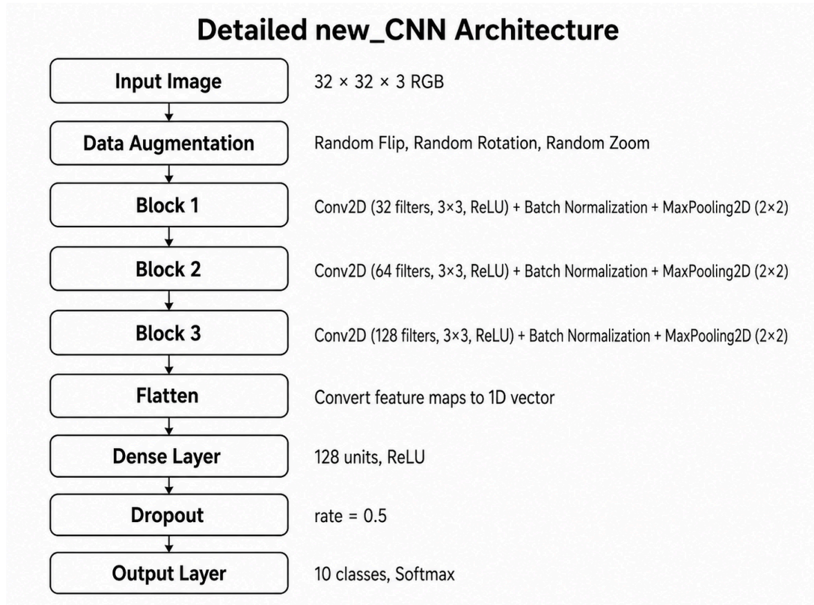
Figure 6.1: new_CNN Architecture
